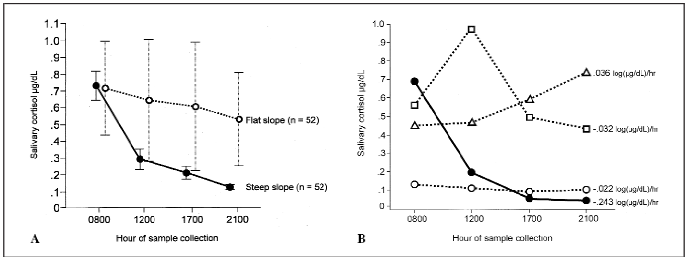
Fig. 1. Panel A: Mean (bars show 95% confidence intervals) diurnal salivary cortisol levels at four times of day for two equal groups of patients split at the median diurnal cortisol slope ( -0.091 \log [\mu\text{g}/\text{dL}] per hour). The average value of the diurnal cortisol slope for the flat slope was -0.040 \log(\mu\text{g}/\text{dL})/\text{hour} and for the steep slope group it was -0.128 \log(\mu\text{g}/\text{dL})/\text{hour} . Panel B: Mean salivary cortisol levels at four times of day, with the diurnal cortisol slope shown in the legend for each plot. Data from four study participants with cortisol profiles that represent the several types of profiles observed. The data from patients who were
